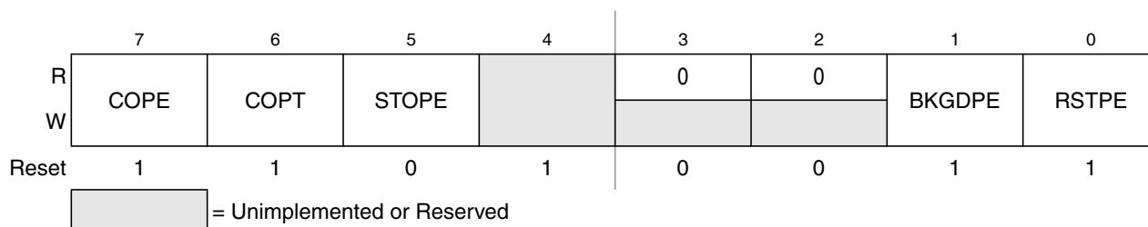
Figure 5-5. System Options Register (SOPT)
