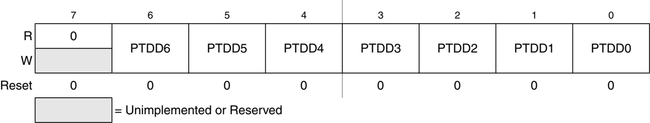
Figure 6-15. Port D Data Register (PTDD)
