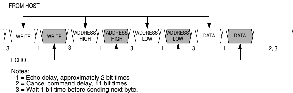
Figure 20-14. Write Transaction
