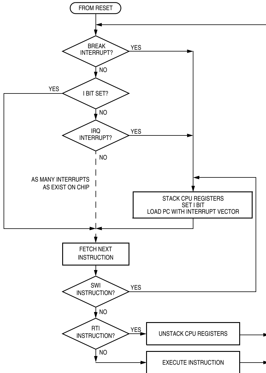
Figure 16-10. Interrupt Processing
