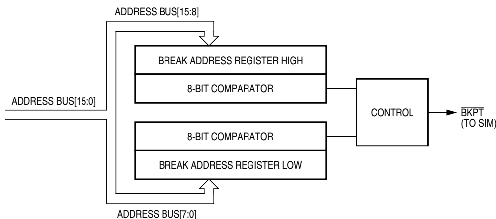
Figure 18-2. Break Module Block Diagram
