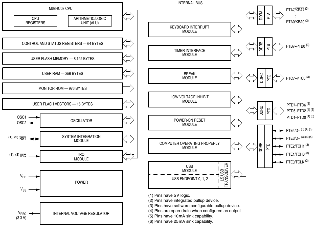
Figure 1-1. MCU Block Diagram
