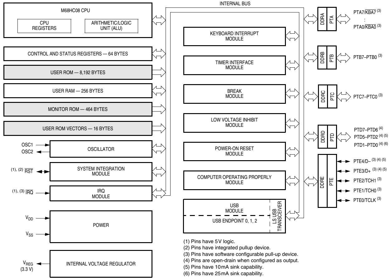
Figure A-1. MC68HC08JB8 Block Diagram
