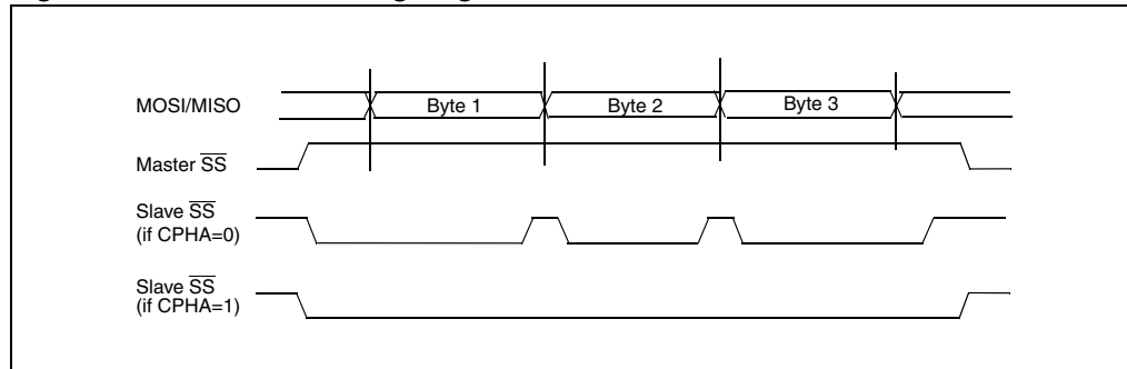
Figure 53. Hardware/software slave select management
