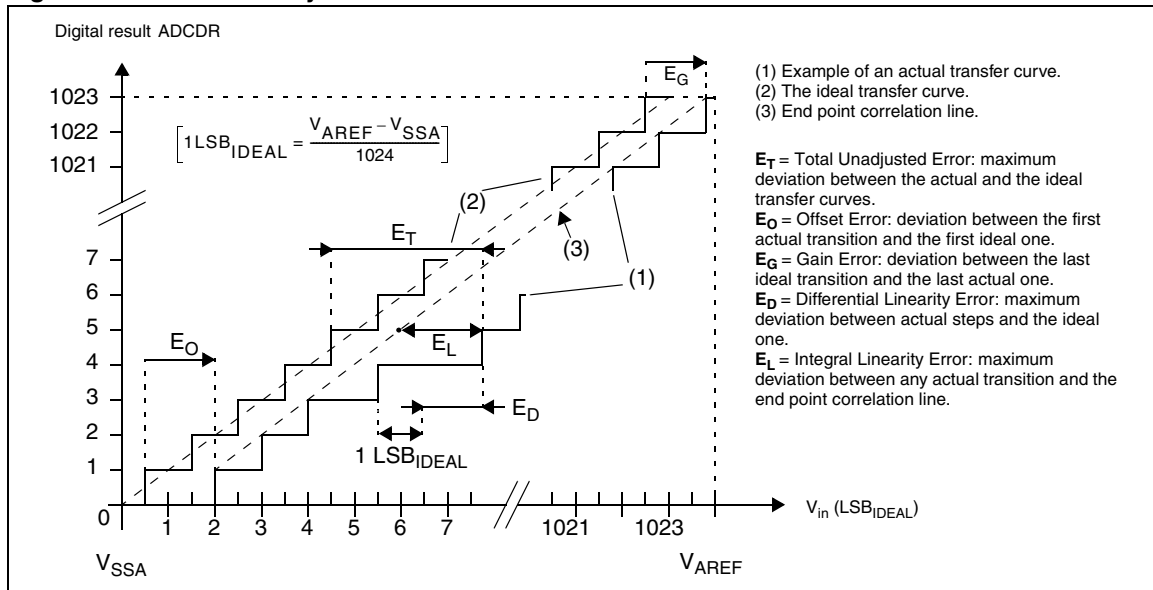
Figure 86. ADC accuracy characteristics
