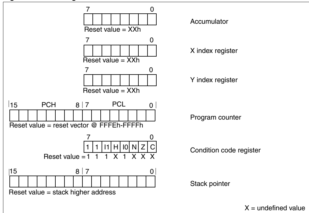
Figure 7. CPU registers
