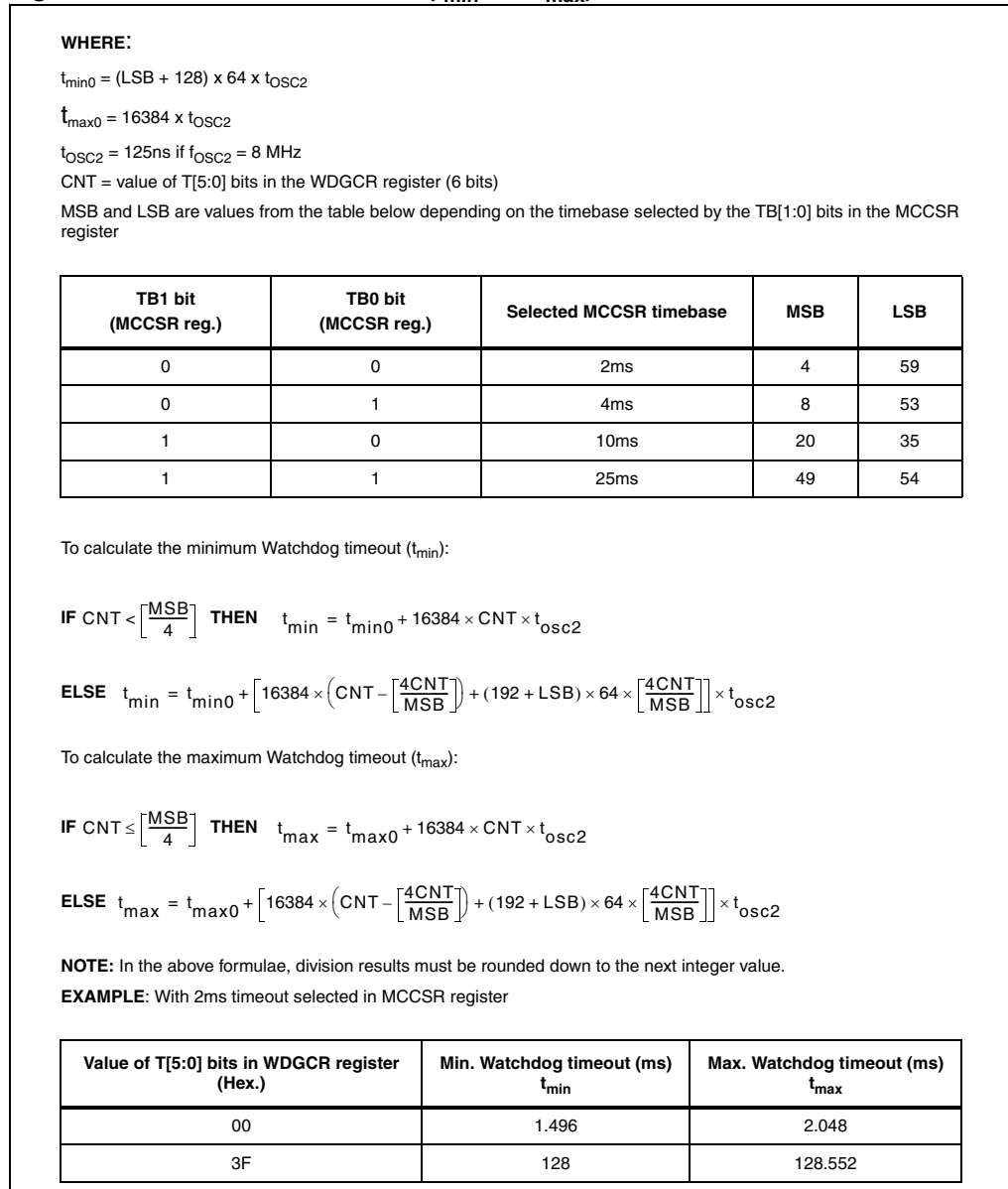
Figure 32. Exact timeout duration ( t_{\min} and t_{\max} )
