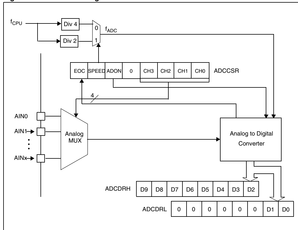
Figure 59. ADC block diagram
