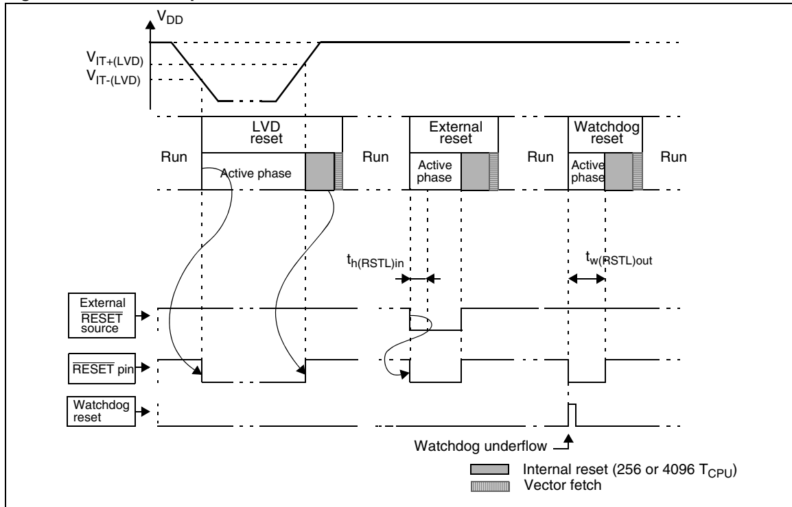
Figure 13. RESET sequences
