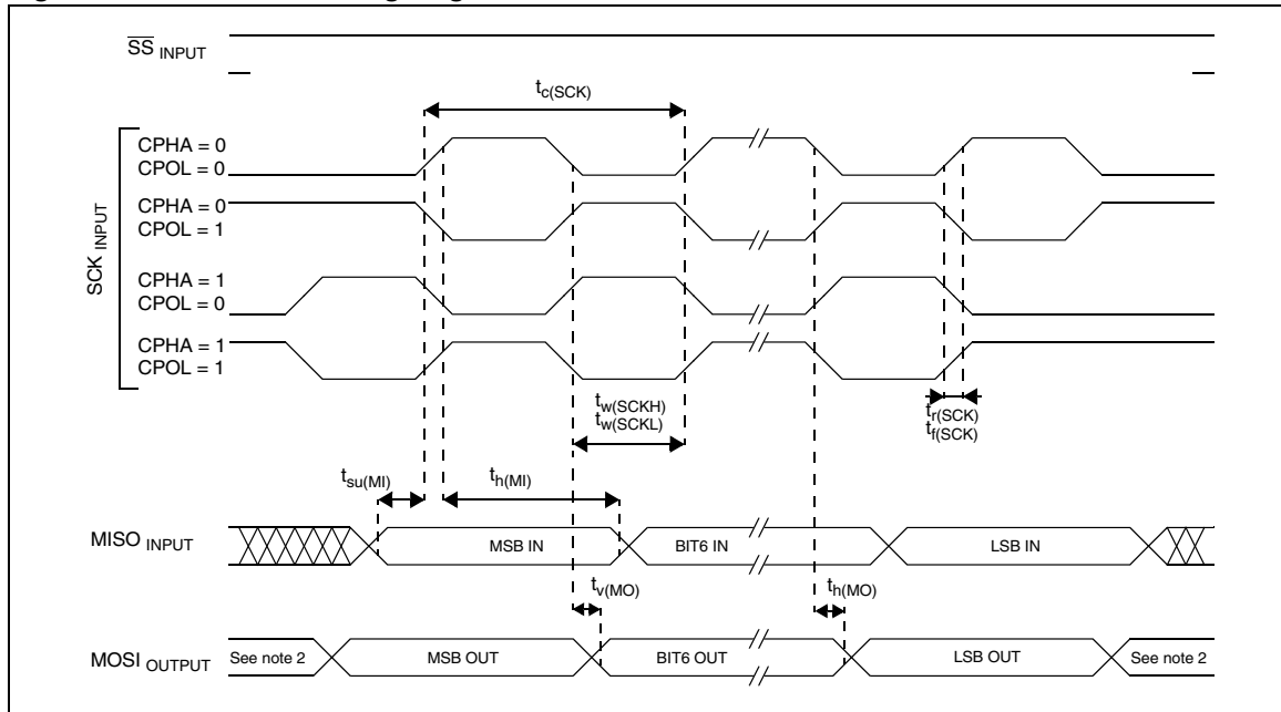
Figure 81. SPI master timing diagram (1)
