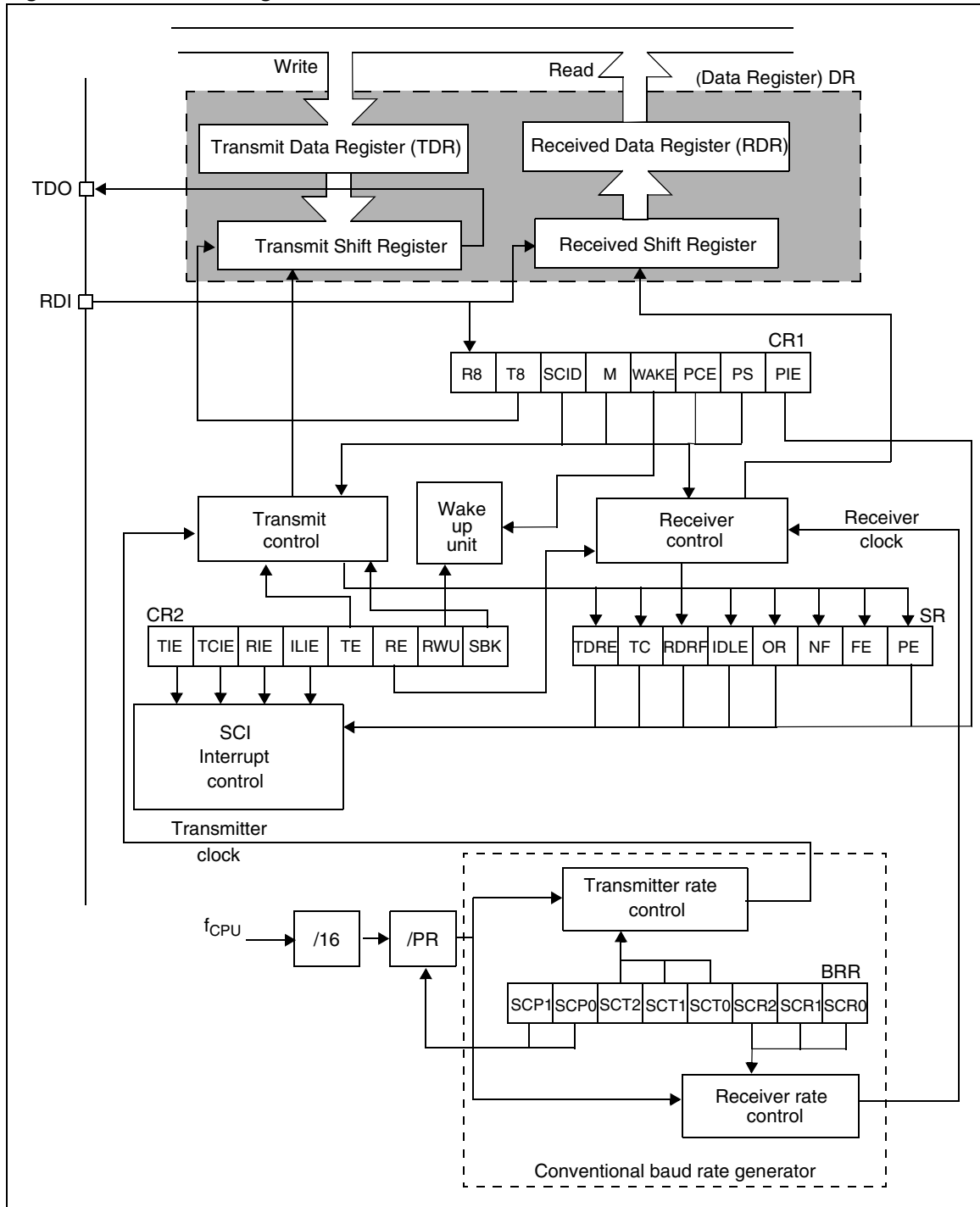
Figure 55. SCI block diagram
