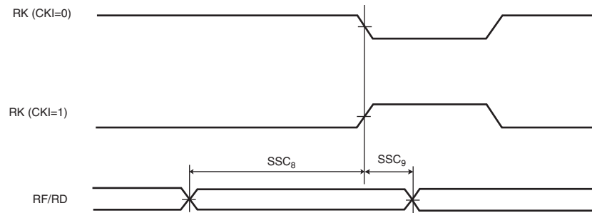
Figure 44-13. SSC Receiver RK and RF in Input
