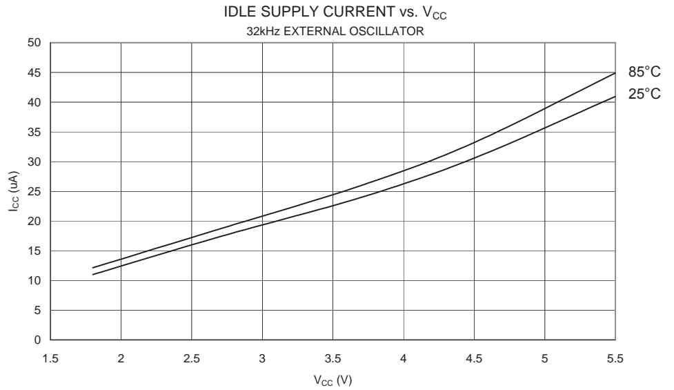
Figure 146. Idle Supply Current vs. V_{CC} (32 kHz External Oscillator)
