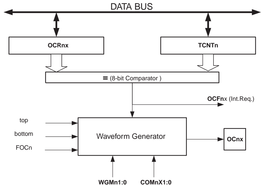
Figure 54. Output Compare Unit, Block Diagram
