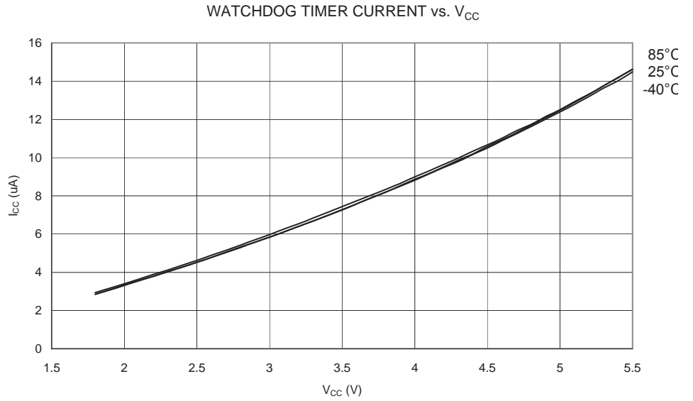
Figure 196. Watchdog Timer Current vs. V_{CC}
