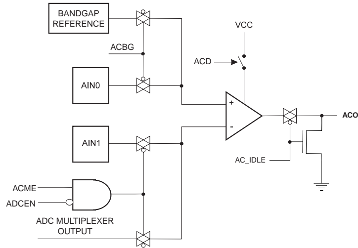
Figure 112. Analog Comparator
