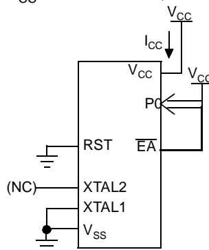
Figure 48. I_{CC} Test Condition, Power-down Mode
