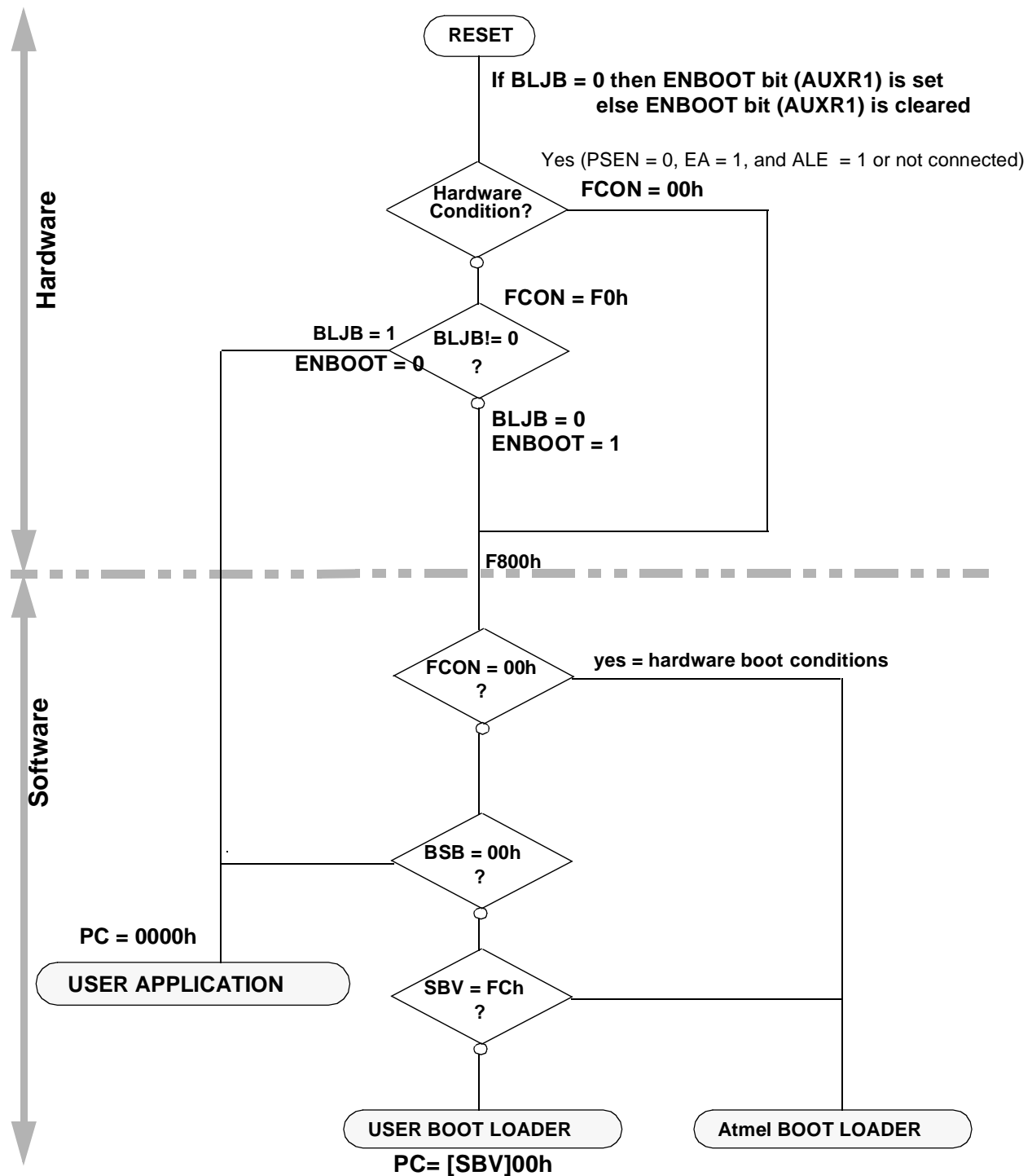
Figure 39. Bootloader process
