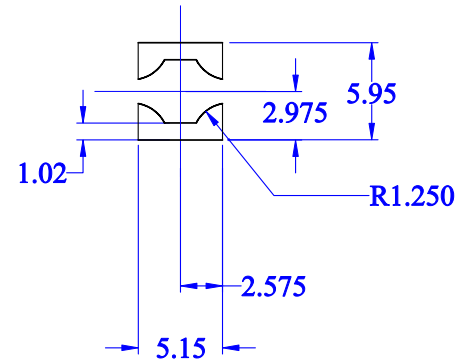
2 PAD LAYOUT
