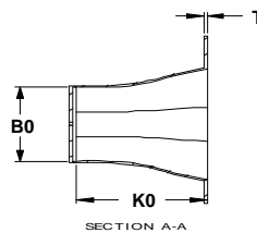
FIGURE 1 CARRIER TAPE & PART
