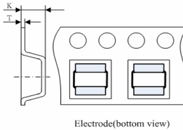
Electrode(bottom view)
