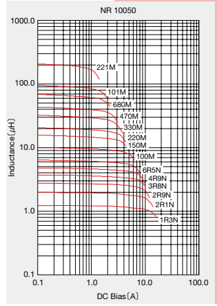
DC Bias characteristics (Measured by HP4285A)
