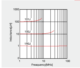
■ Inductance-vs-Frequency characteristics
