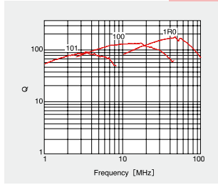
■ Q-vs-Frequency characteristics
