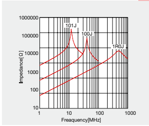
■ Impedance-vs-Frequency characteristics
