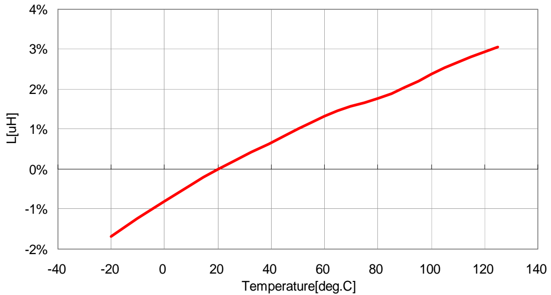
VLF4014ST-6R8M2R2
