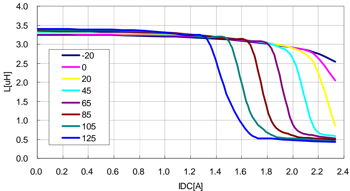
VLF4014ST-4R7M1R4
