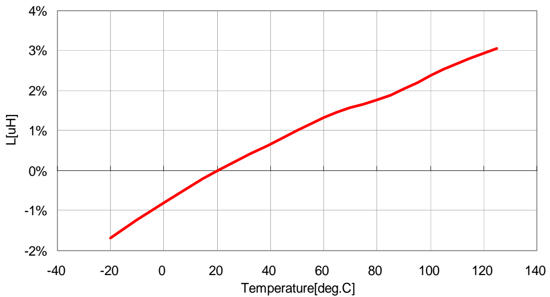
VLF4014ST-4R7M1R4
