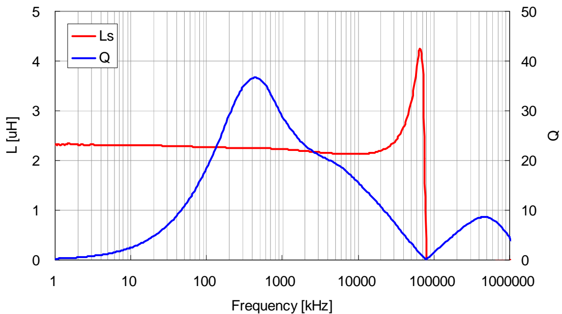
VLF4014ST-2R2M1R9
