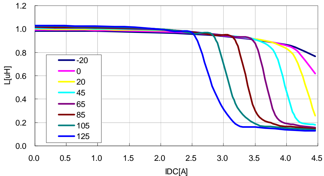
VLF4014ST-1R0N2R3
