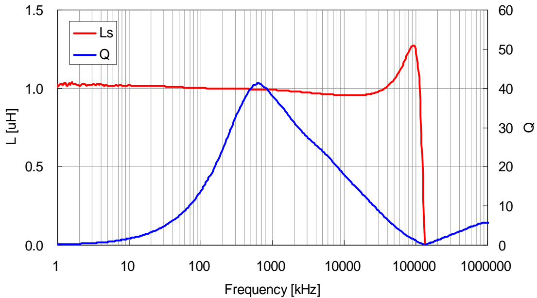
VLF4014ST-1R0N2R3
