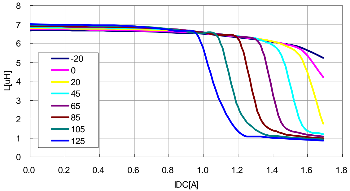
VLF4014ST-6R8M2R2
