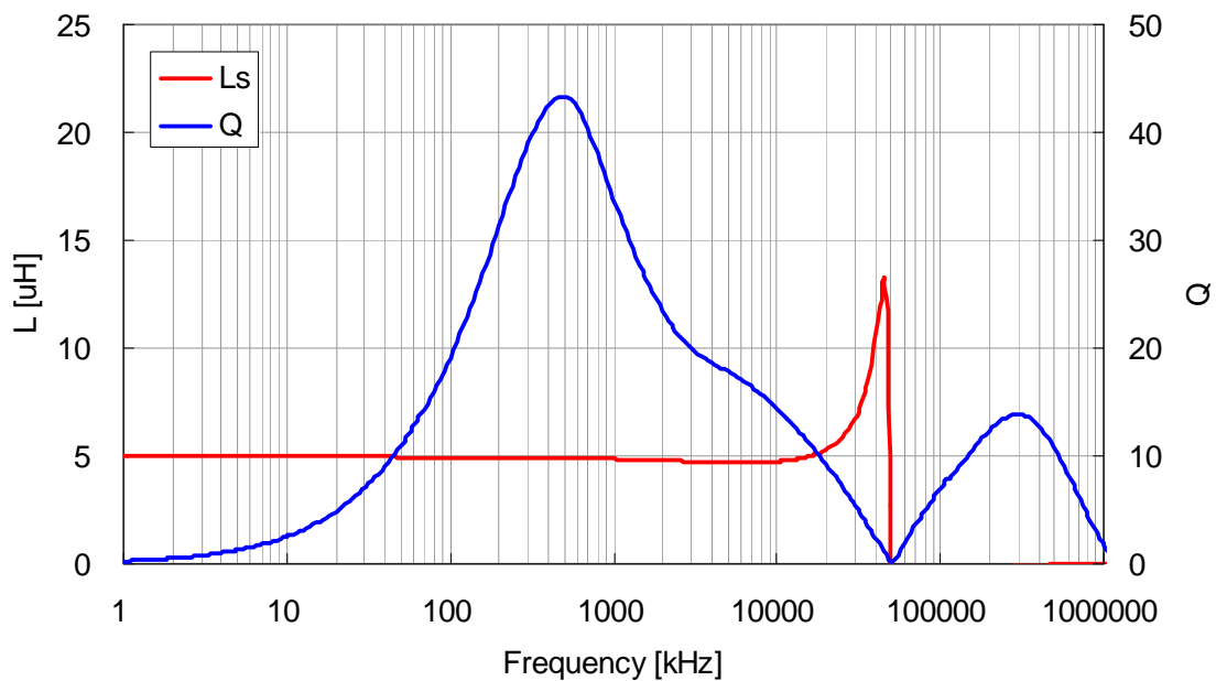
VLF4014ST-4R7M1R4
