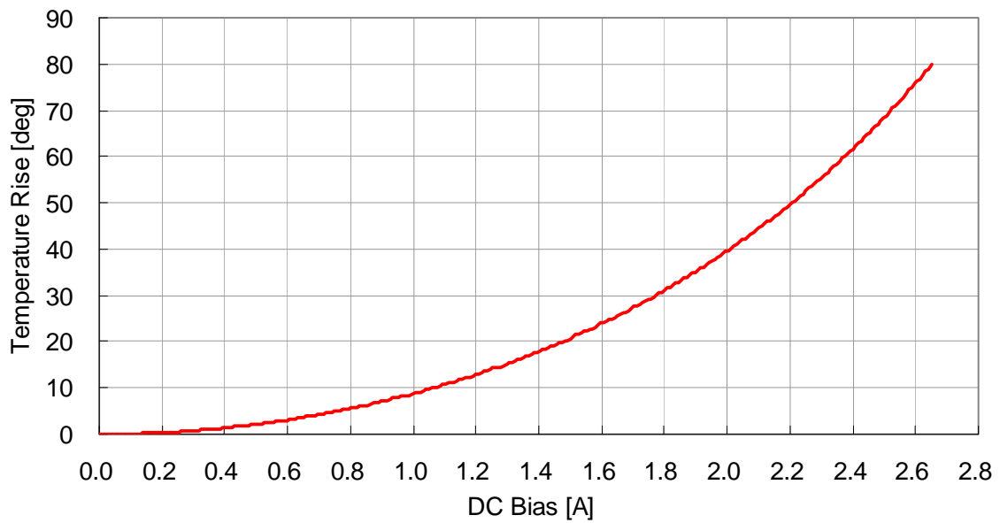
VLF4014ST-2R2M1R9
