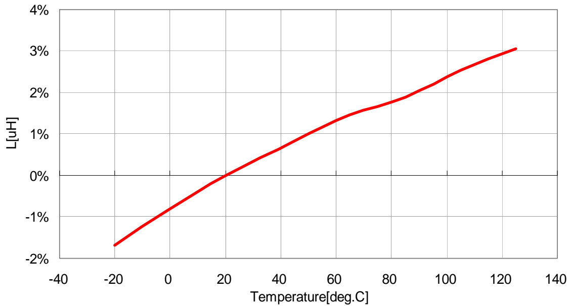
VLF4014ST-1R0N2R3
