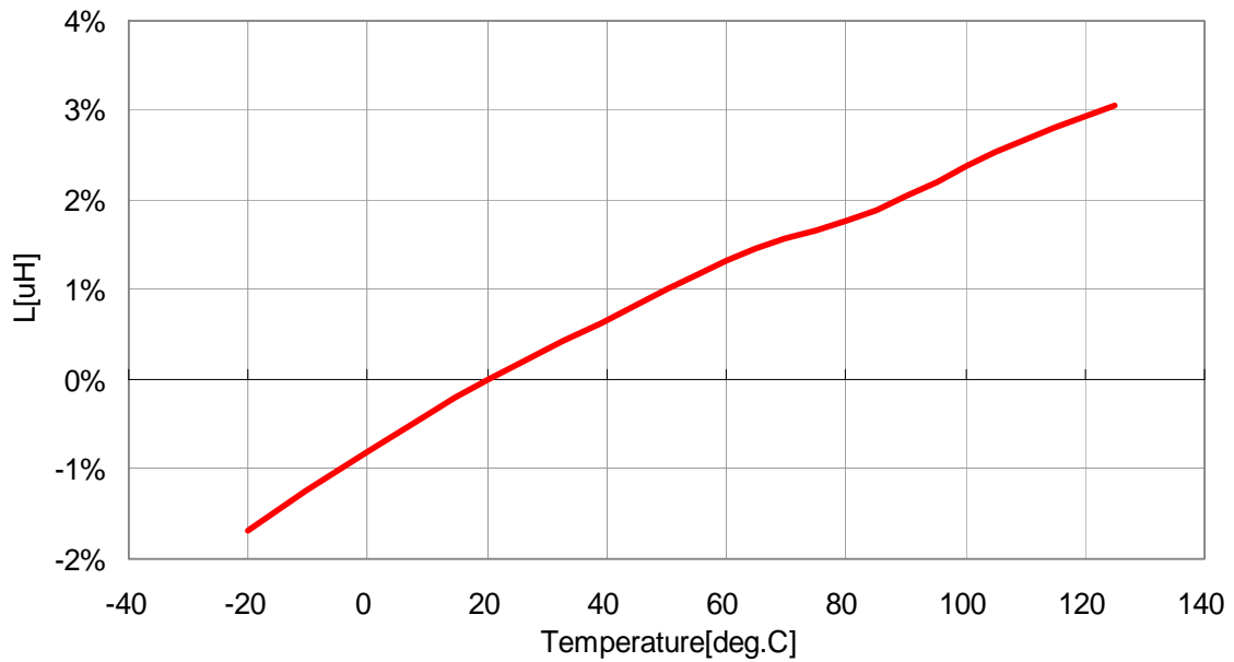
VLF4014ST-3R3M1R6
