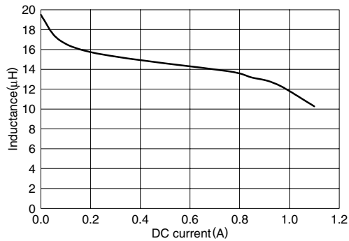
VLF5014AT-150MR76
