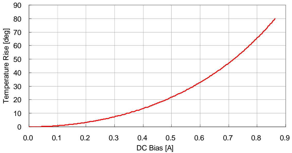
VLS3012T-330MR40
