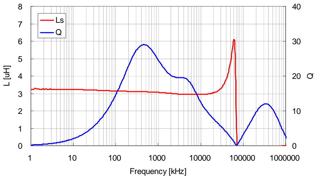
VLS3012T-3R3M1R3
