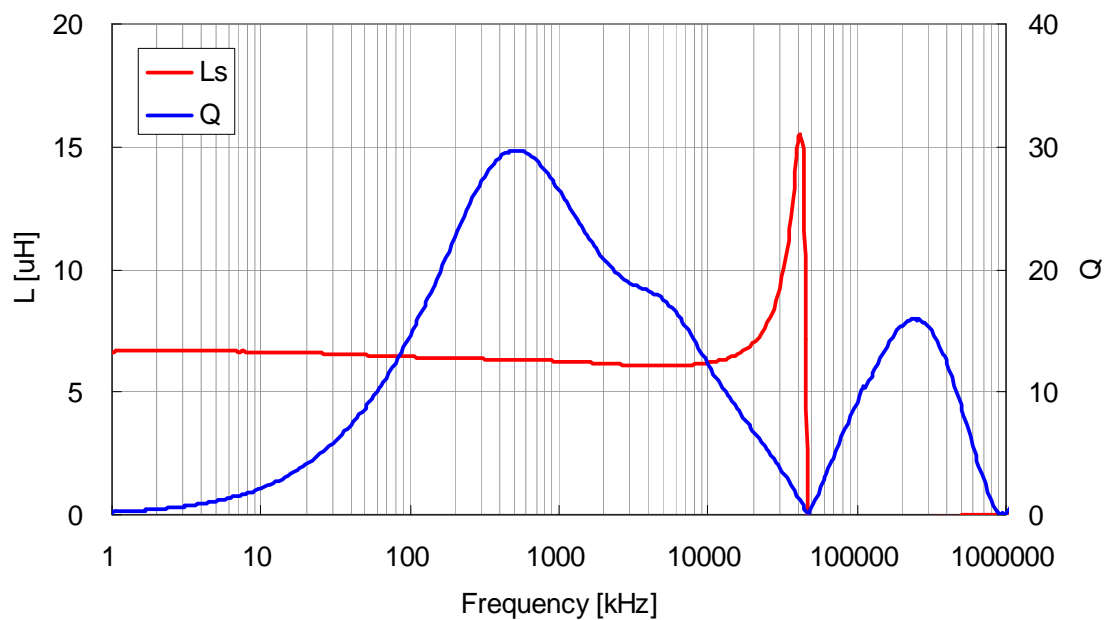
VLS3012T-6R8MR90
