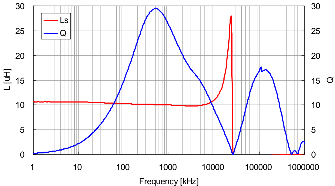
VLS3012T-100MR72
