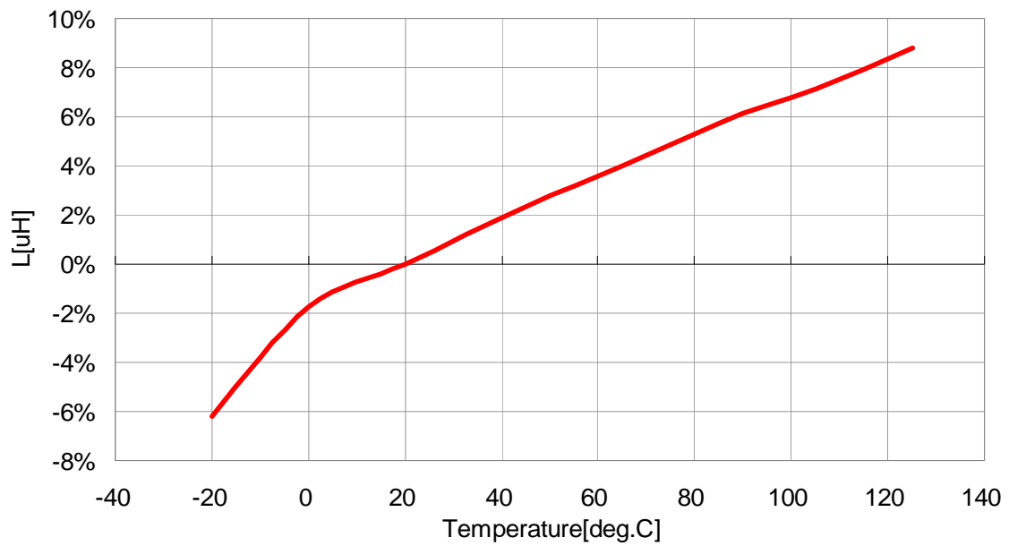
VLS3012T-330MR40
