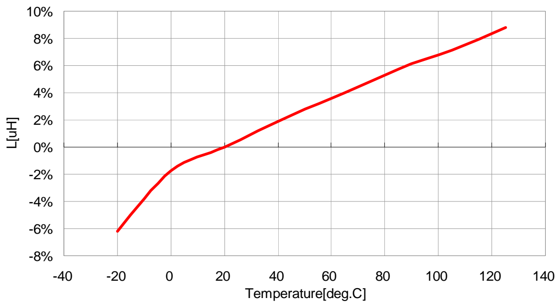
VLS3012T-3R3M1R3
