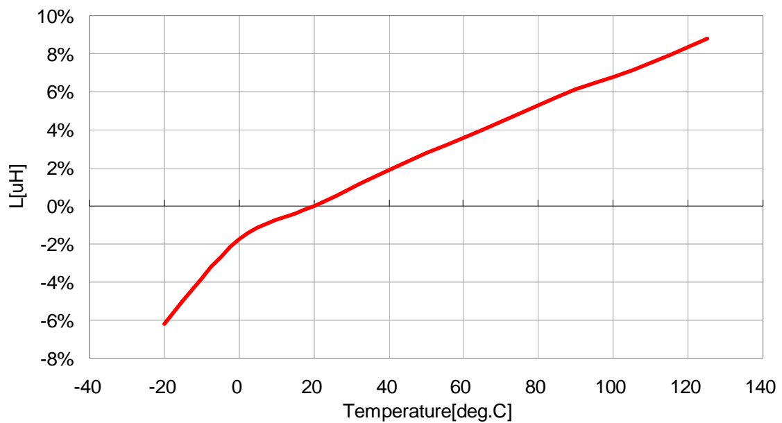
VLS3012T-150MR58
