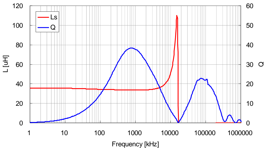
VLS3012T-330MR40
