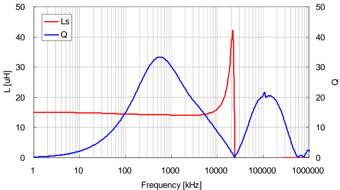
VLS3012T-150MR58
