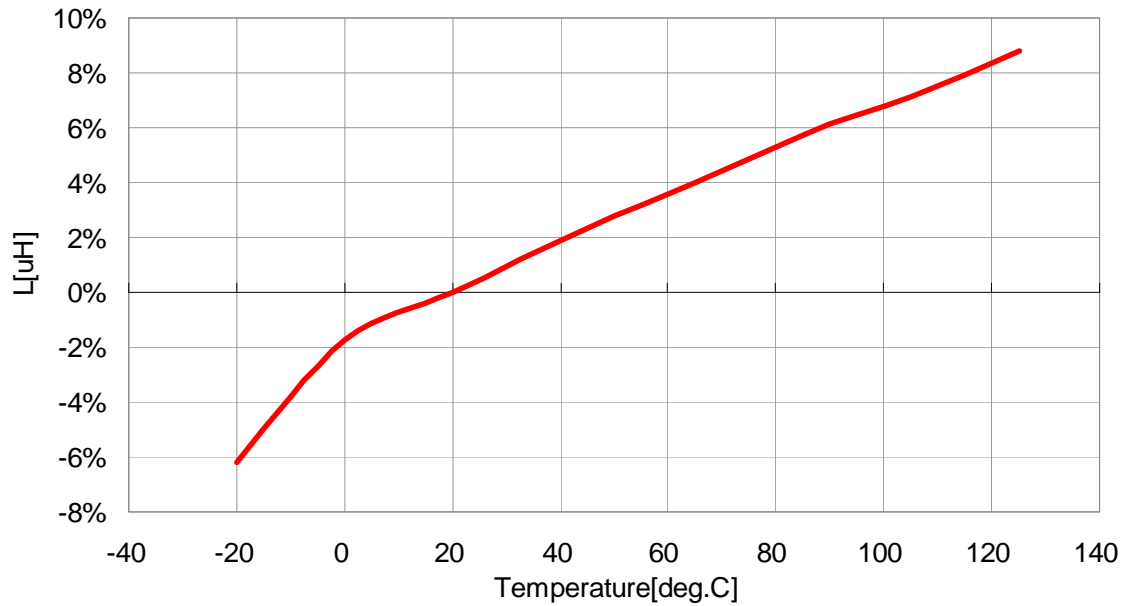
VLS3012T-100MR72
