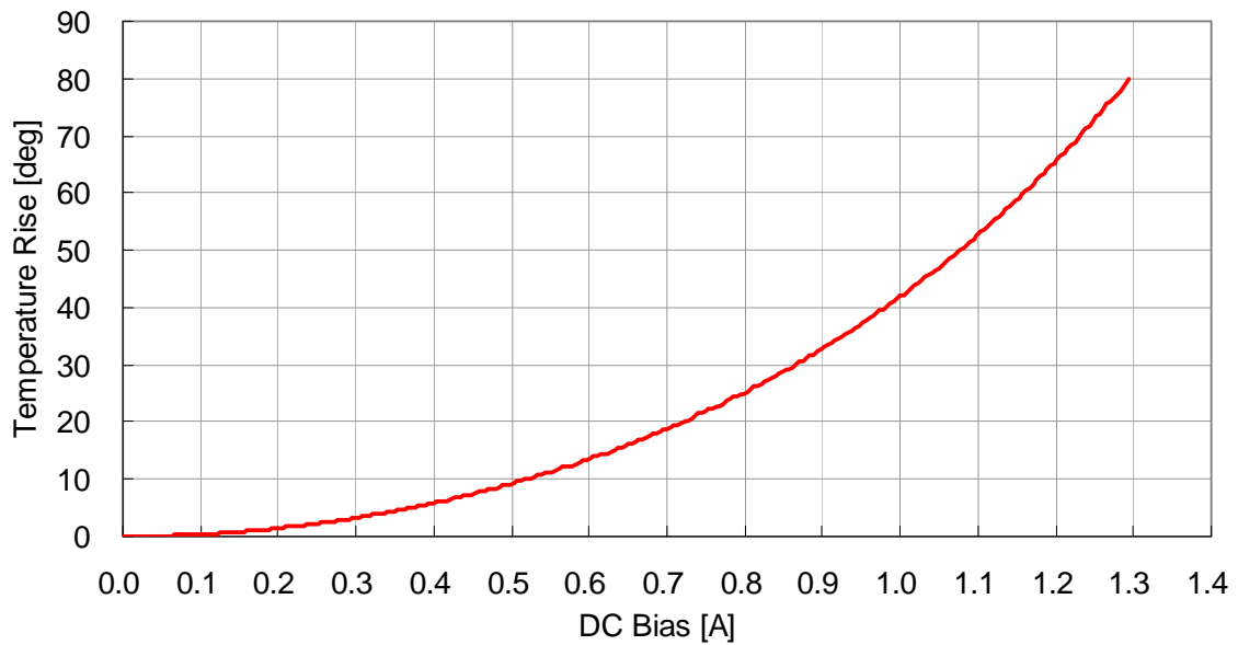
VLS3012T-150MR58
