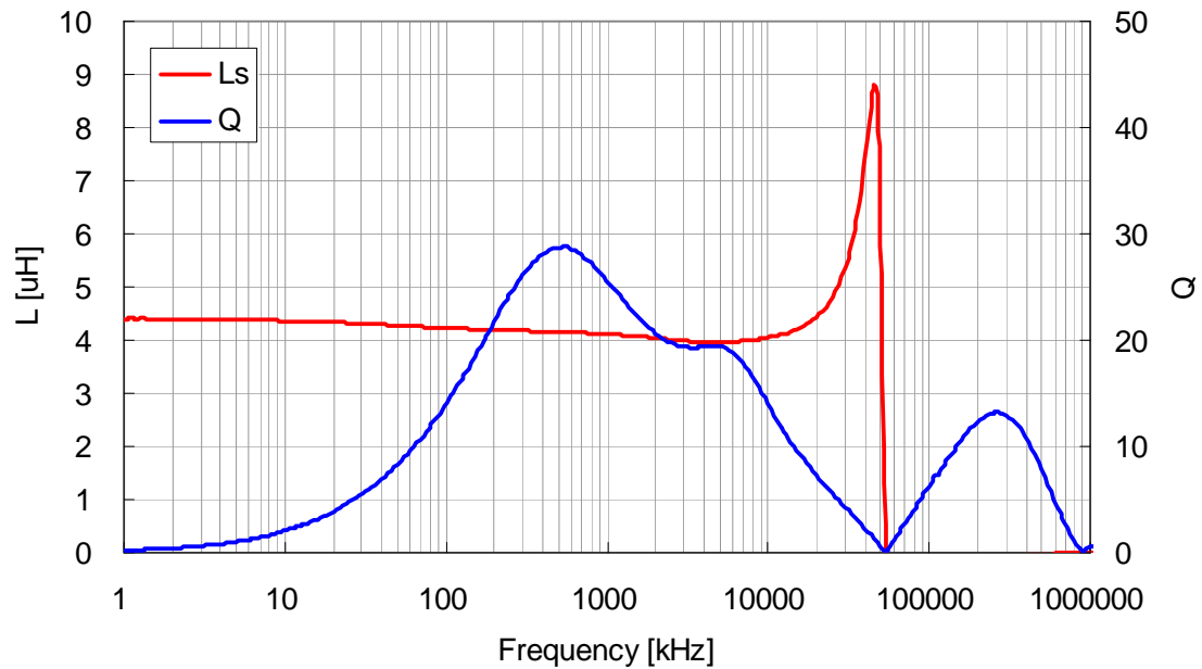
VLS3012T-4R7M1R0
