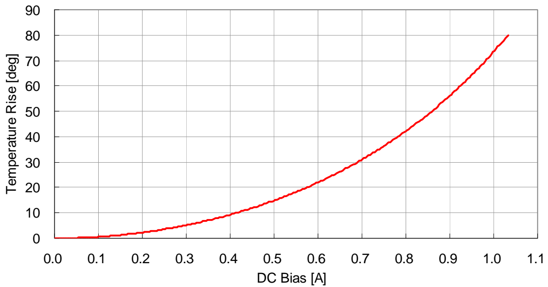
VLS3012T-150MR58
