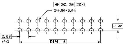
RECOMMENDED PCB PATTERN
