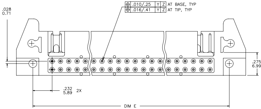
VIEW F-F
