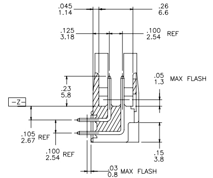
SECTION G-G ROTATED 90° CW
