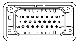
776228-5 & 1-776228-5 KEY LOCATION SCALE 2:1
