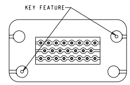
KEYING FOR 776228-2 AND 776228-4 SCALE 2:1
