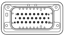
776228-4 & 1-776228-4 KEY LOCATION SCALE 2:1
