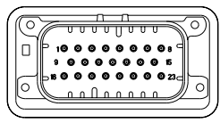
776228-2 & 1-776228-2 KEY LOCATION SCALE 2:1
