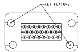
KEYING FOR 776228-1 AND 776228-5 SCALE 2:1
