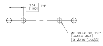
RECOMMENDED BOARD LAYOUT
