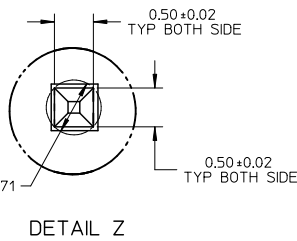
DETAIL Z
