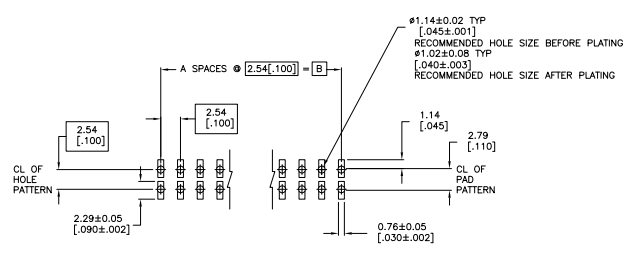
RECOMMENDED PC BOARD MOUNTING DIMENSIONS FOR .063 [1.60] THICK PC BOARD AND .012 [1.305] STENCIL THICK.
