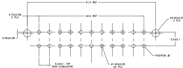
COMPONENT SIDE SHOWN RECOMMENDED MOUNTING HOLE PATTERN FOR 1.78 MAX THICK P.C. BOARD
