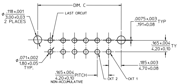
LAYOUT FOR 4-24 CIRCUIT
