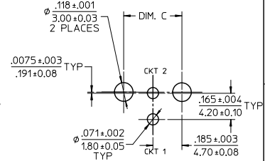
LAYOUT FOR 2 CIRCUIT
