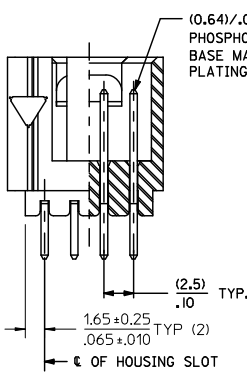
SECTION E-E
