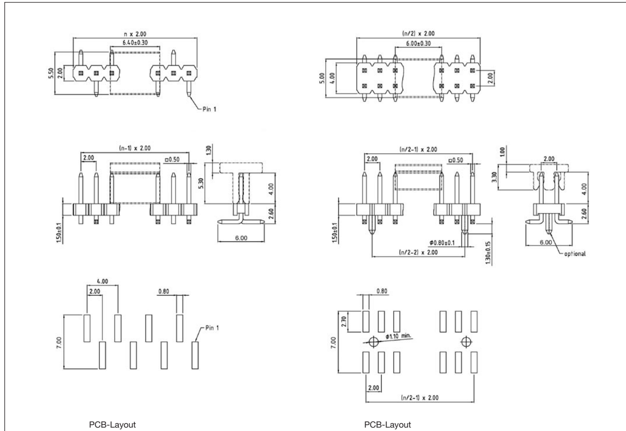
PCB-Layout
