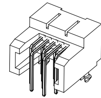
ISOMETRIC VIEW SCALE 3:1
