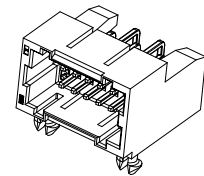
ISOMETRIC VIEW SCALE 3:1
