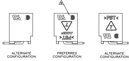
POSSIBLE MARKING CONFIGURATIONS SCALE 5:1
