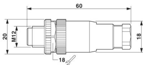
M12 x 1 male connector, straight
