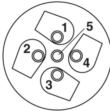
Cable connection side M12 (screw connection) Pin assignment M12 male connector, 5-pos., A-coded, male side
