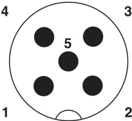
Male/Female M12
