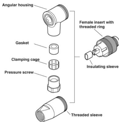
Male/Female M12
