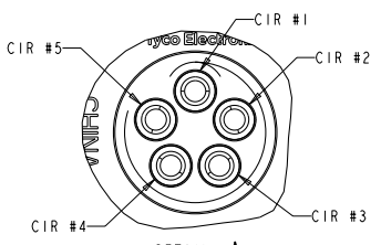
DETAIL A CIRCUIT DESIGNATION VIEW SCALE 8:1
