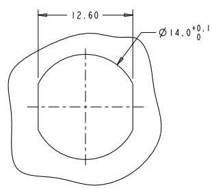
SUGGESTED PANEL CUTOUT SCALE 4:1
