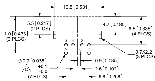
HOLE LAYOUT TOP VIEW
