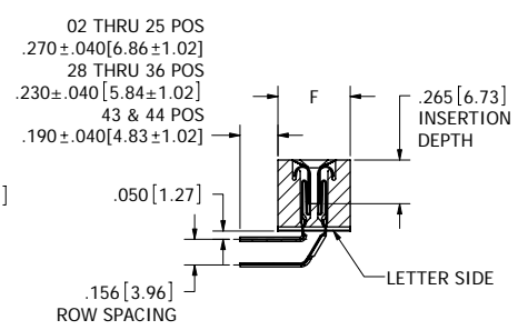
CONTACT ID SCALE 3:1 (PINS OMITTED FOR CLARITY)
