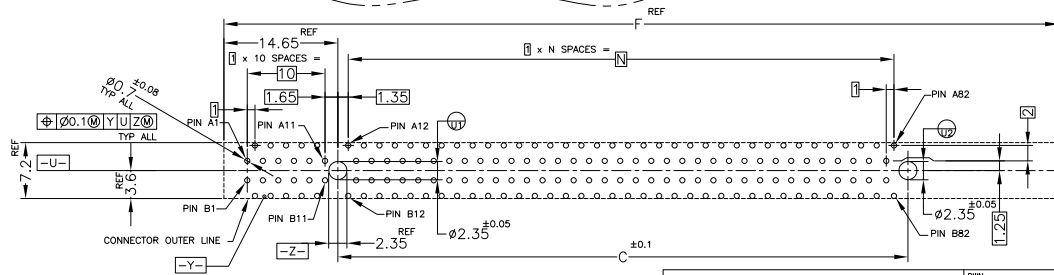
PCB PATTERN LAYOUT
