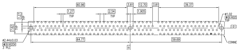
RECOMMENDED PCB LAYOUT (TOP VIEW) TOLERANCE : ±0.05
