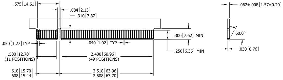
DAUGHTER CARD LAYOUT
