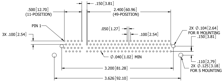
RECOMMENDED PCB LAYOUT, COMPONENT SIDE
