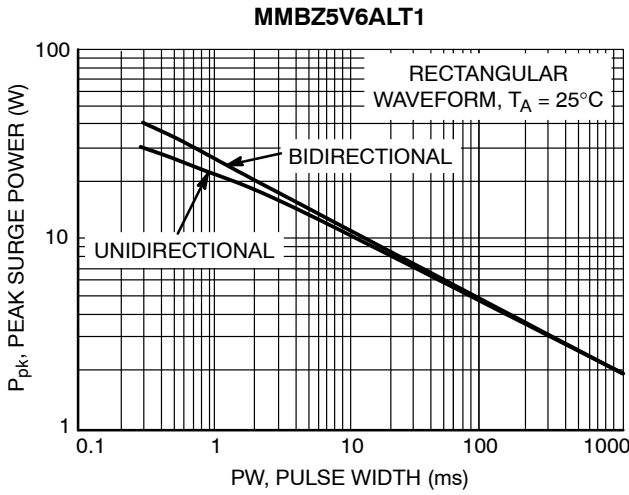
Figure 8. Maximum Non-repetitive Surge Power, P_{pk} versus PW
