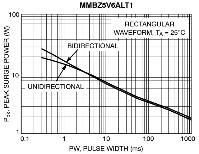
Figure 9. Maximum Non-repetitive Surge Power, P_{pk(NOM)} versus PW
