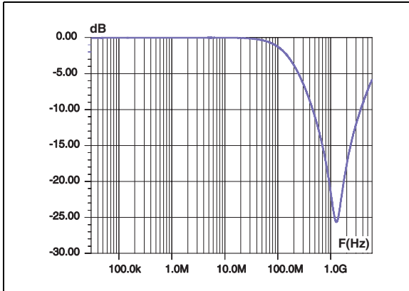
Figure 9. S21 attenuation measurement results of each channel
