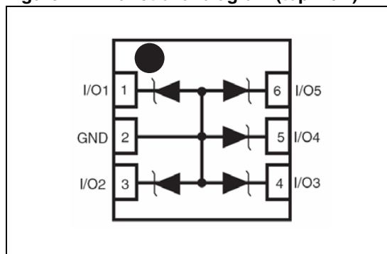
Figure 1. Functional diagram (top view)
