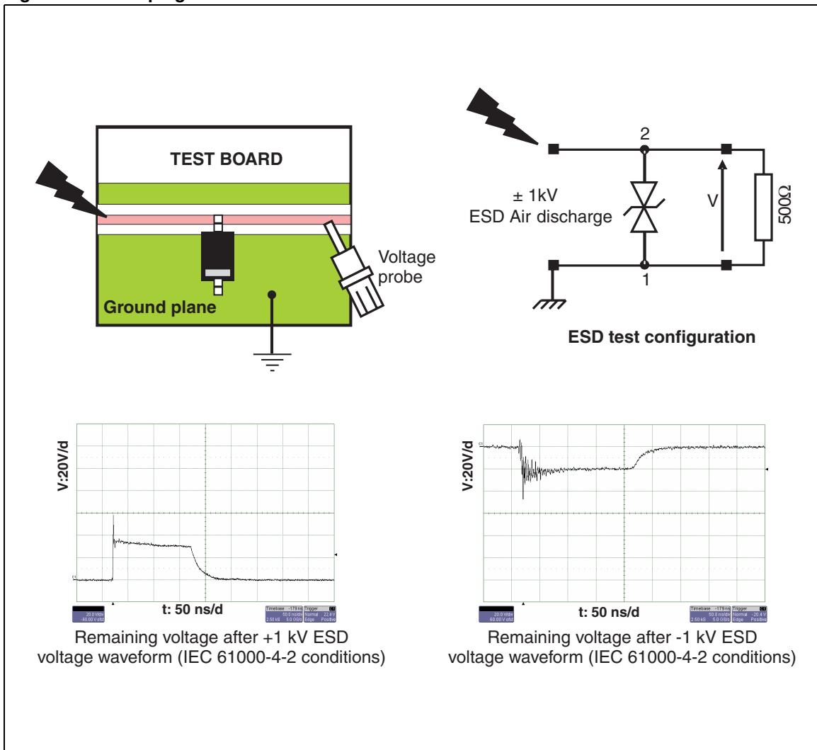
Figure 5. Clamping test conditions and results
