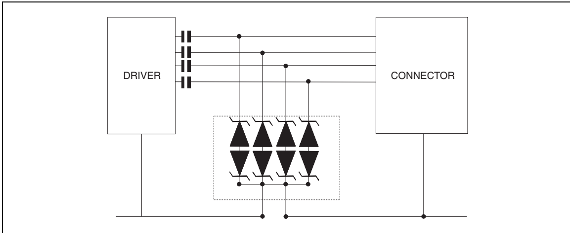
Figure 7: Bidirectional protection for 0V biased signals
