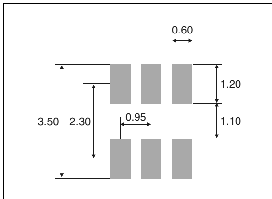
Figure 10: Foot Print Dimensions (in millimeters)
