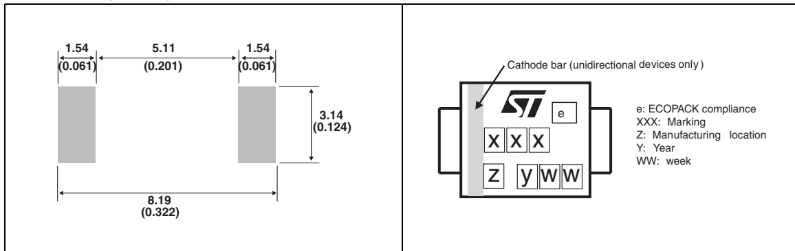
Figure 13. SMC footprint dimensions in mm (inches)
