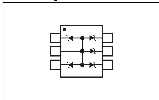
Figure 1. ESDALC6V1-5P6 functional diagram
