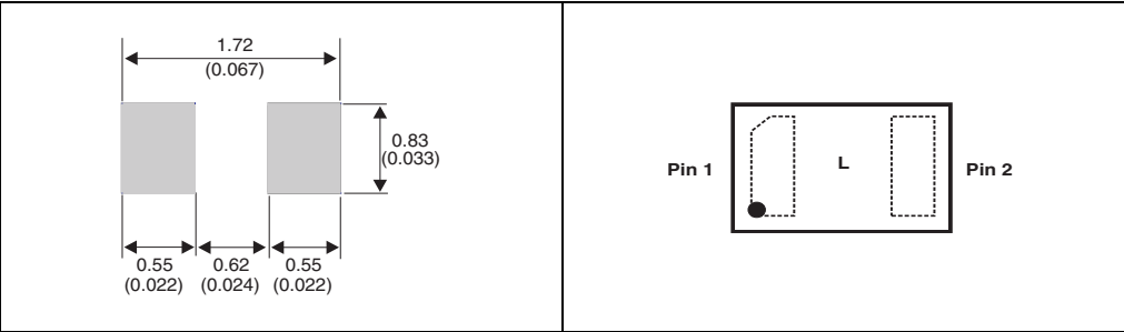
Figure 11. Footprint dimensions in mm (inches)
