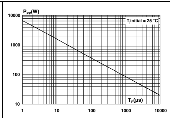
Figure 5. Peak pulse power versus exponential pulse duration
