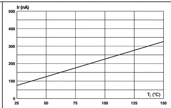
Figure 9. Leakage current versus junction temperature (typical values)
