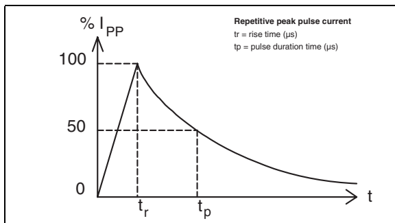
Figure 1. Pulse waveform (10/1000 \mu s )
