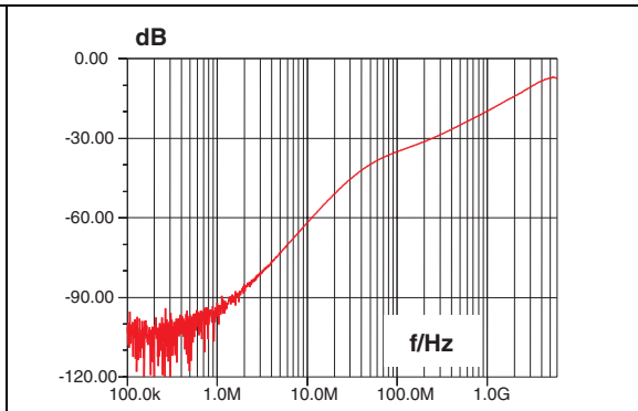
Figure 9. Analog crosstalk measurements between channels
