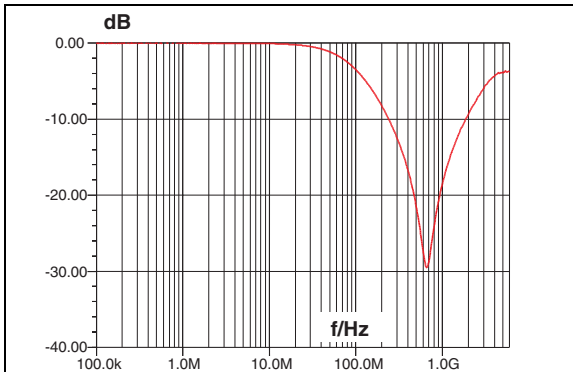
Figure 8. S21 attenuation measurement results of each channel
