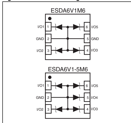
Figure 1. Functional diagram
