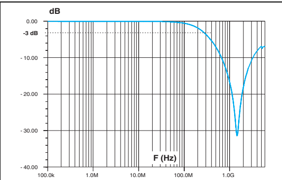
Figure 10. S21 attenuation measurement result
