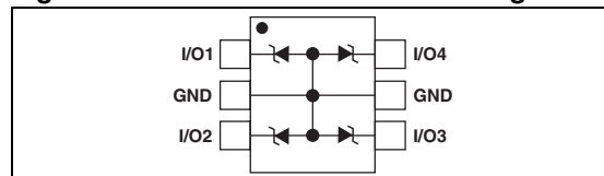
Figure 1. ESDA6V1P6 functional diagram
