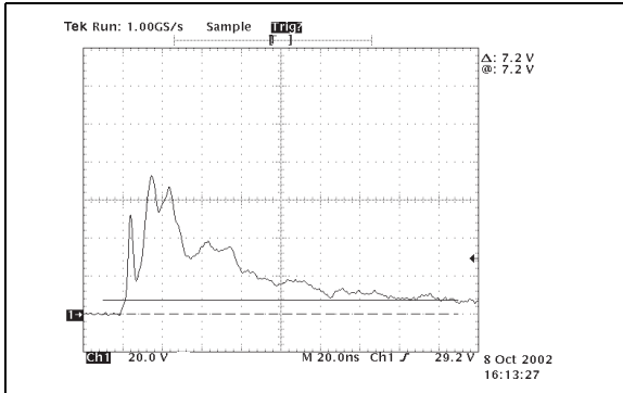
Figure 10. ESD response @ V_{PP} = 15 kV air discharge (ESDA6V1-5P6)
