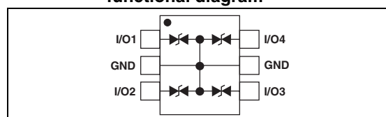
Figure 3. ESDA14V2BP6 and ESDA25-4BP6 functional diagram
