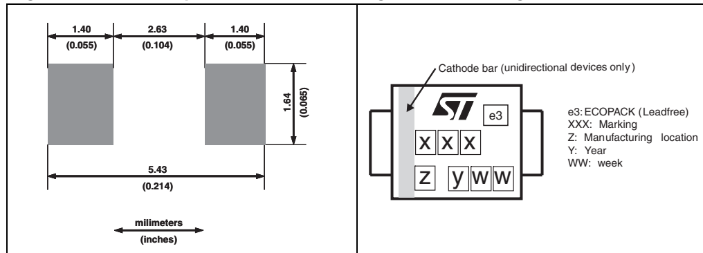
Figure 11. SMA footprint dimensions
