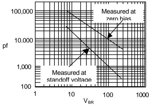
Typical Capacitance (pf) – versus – Breakdown voltage
