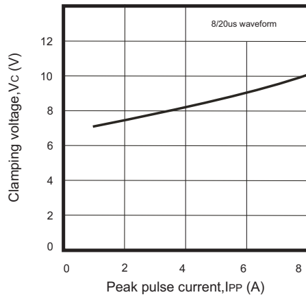
Fig. 3 - Clamping volatage vs. peak pulse current
